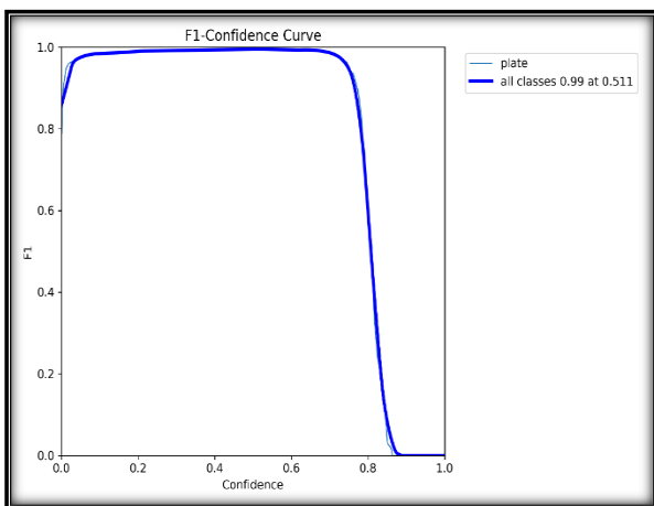
Figure 13: F1-Confidence Curve for the Detection Model
