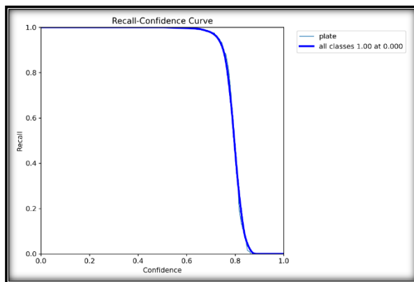
Figure 18: The Recall-Confidence Curve of the Detection Model
