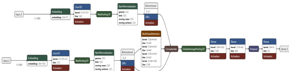
Figure 2: Proposed Hybrid Model of CNN and GRUs.
