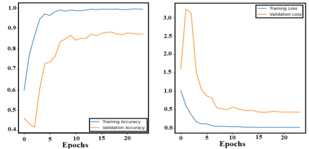
EfficientNetB0
