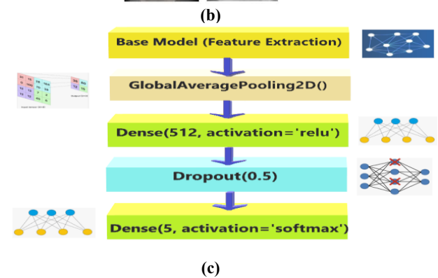
Figure 3: The proposed methodology: (a) The general steps, (b) the data preprocessing steps on a training sample, (c) The proposed architecture for all DL models.
