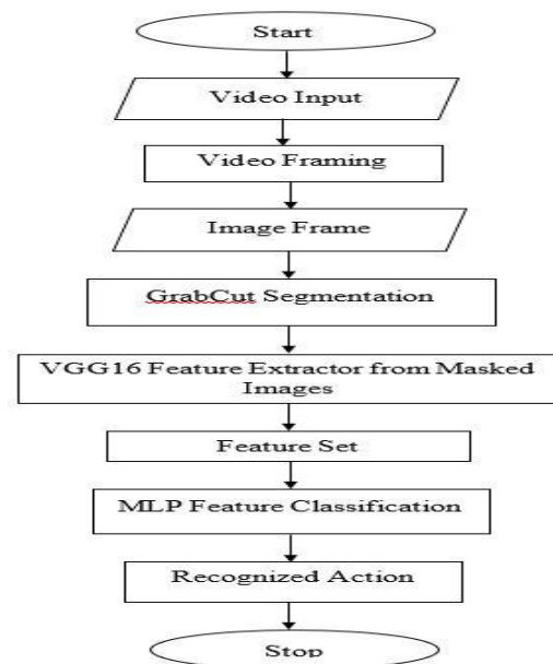
Figure 2: Flowchart of Experimental Pipelin
