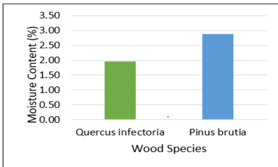
Figure 1: Effect of wood species on Moisture Content
