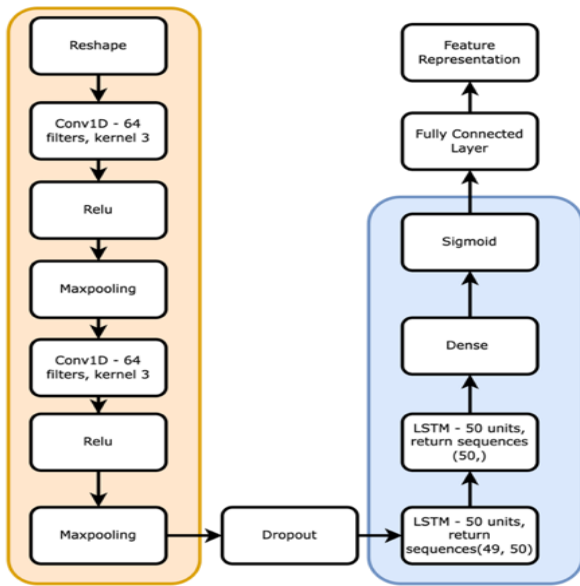
Figure 1: CNN LSTM Architecture
