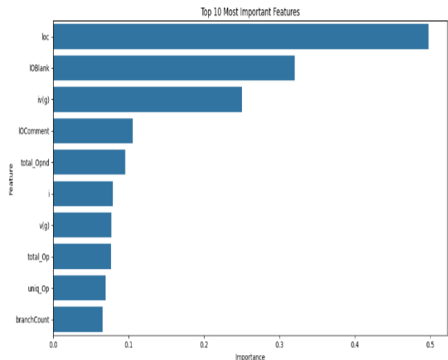
Figure 3: Feature Importance
