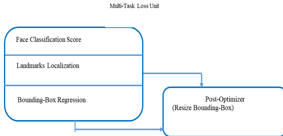
Figure 4: The multi-task loss unit after post-refinement.
