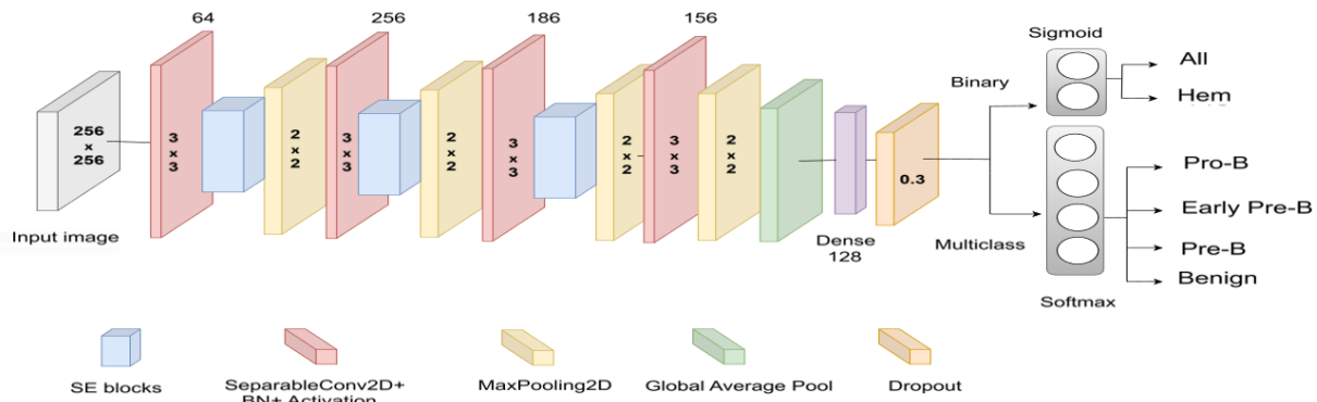
Figure 4: Architecture of the SE-CNN model.
