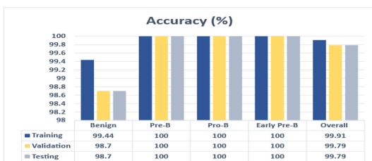
Figure 8: Class-wise and overall accuracy performance of the proposed multi-class classification model.
