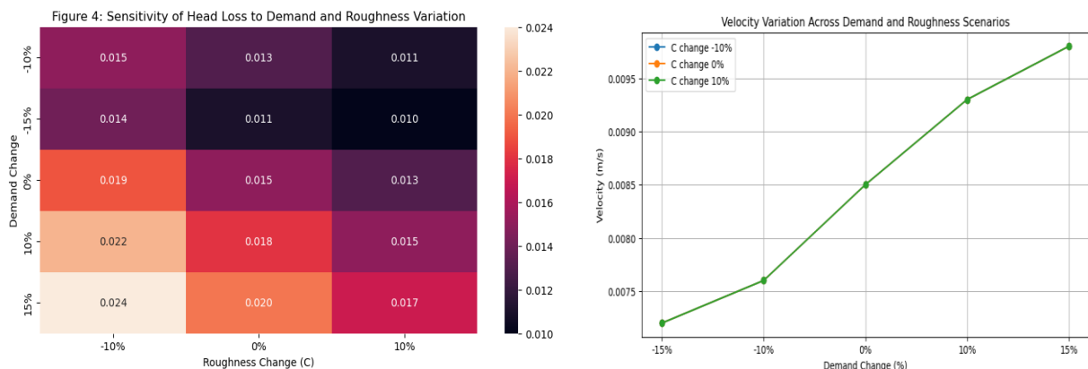
Figure 4: Heatmap and performance trends illustrating the impact of demand and roughness variations on head loss, velocity, and total cost. The optimized design remains feasible and stable across all fifteen sensitivity scenarios.
