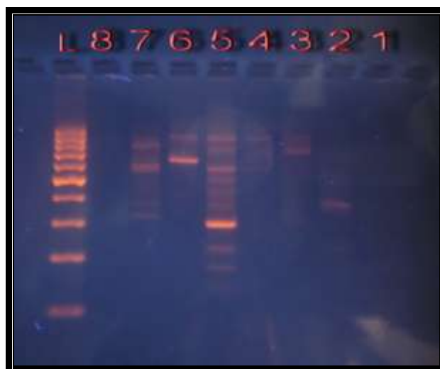
(Figure 1): 1.5 % Agarose gel analysis of PCR profile obtained on Amplification with primers, ITS1F and ITS4, general for higher fungi, (1) P. ostreatus (2) P. sapidus (L) DNA Ladder 100 bp (DNA molecular weight marker).
